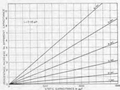
FIGURE 1. Increase in effective capacitance of a precision condenser caused by an equivalent inductance of 0.06 \mu\text{h}
